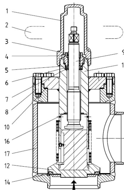
DN 125 – 250
